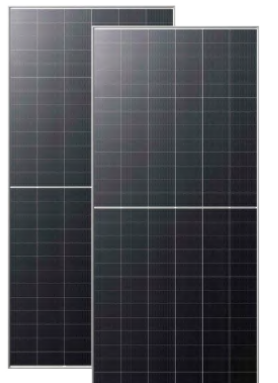
615-635Wp 78HL4 BDV TIGER NEO N-TYPE
